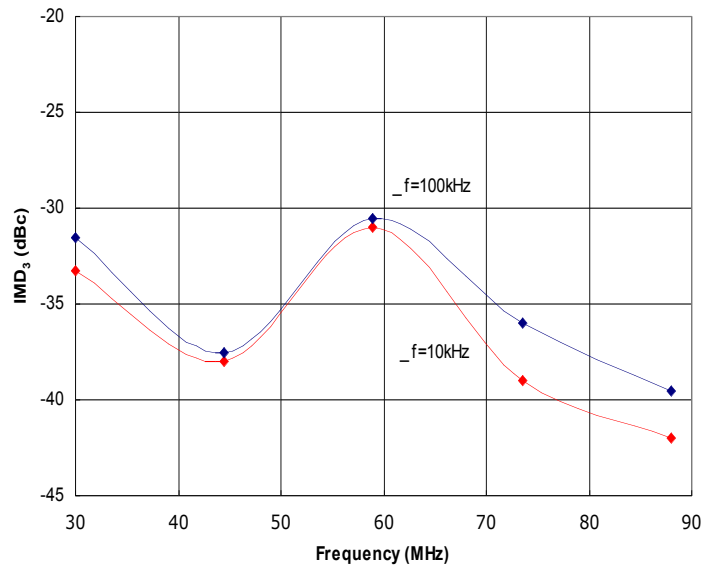
Figure 2: HD30847 Typical IMD 3 , Δf=10kHz and 100kHz, @ P out = 50W PEP. For improved linearity, see our HD30842 Class A amp.
