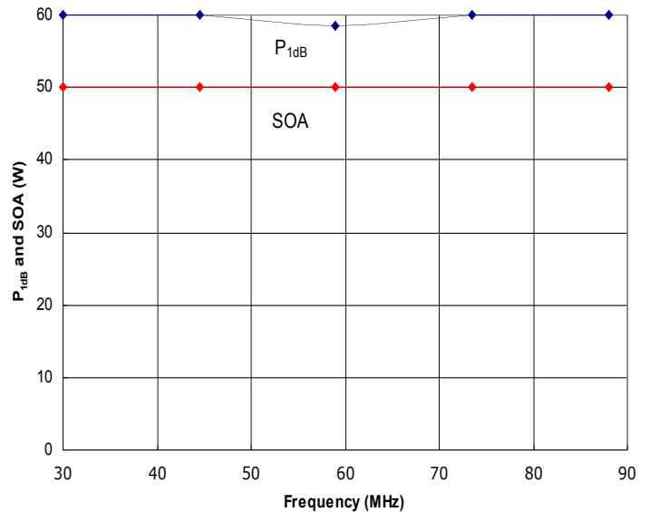
Figure 4: HD30847 Typical P 1dB and Safe Operating Area (SOA).
