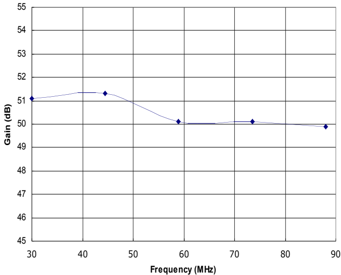
Figure 1: HD30847 Typical Gain @ P out = 50W.
