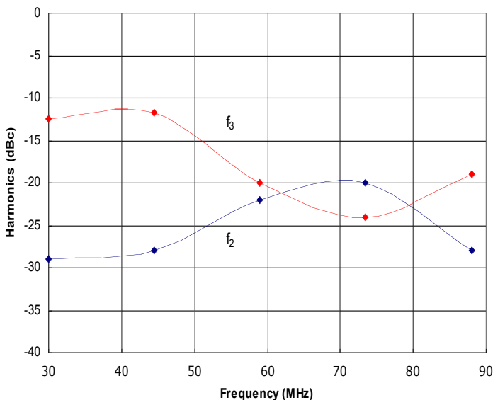
Figure 3: HD30847 Typical f 2 and f 3 @ P out = 50W.
