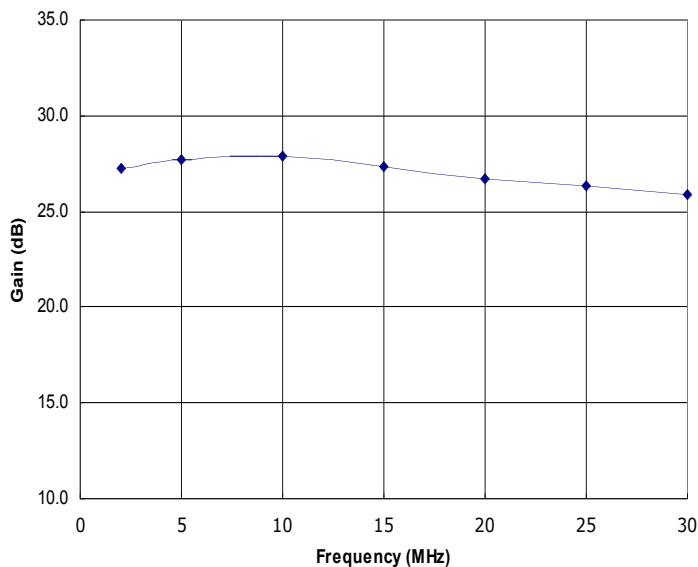
Figure 1: HD30815 Typical Gain @ P_{out} = 500W .
