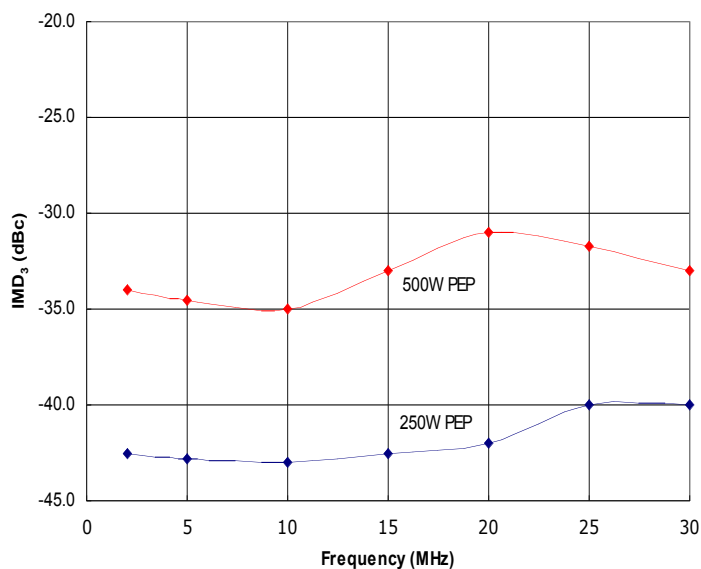
Figure 2: HD30815 Typical IMD 3 @ \Delta f = 10kHz , 500W PEP and 250W PEP.
