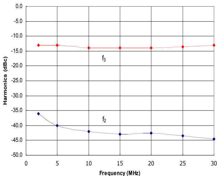
Figure 3: HD30815 Typical f_2 and f_3 @ P_{out} = 500W .
