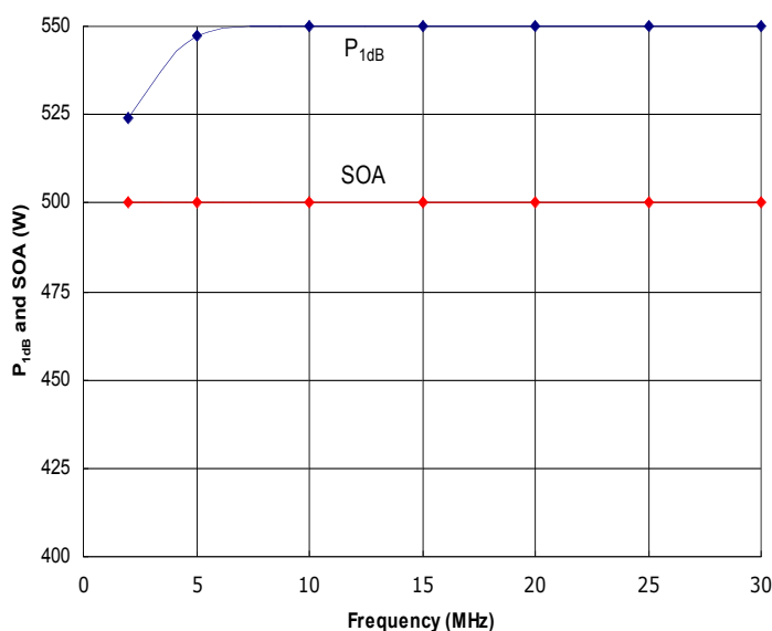
Figure 4: HD30815 Typical P 1dB and Safe Operating Area (SOA). Do not exceed the SOA.
