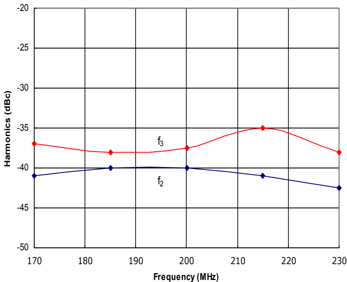
Figure 3: HD30723 Typical f 2 and f 3 @ P out = 25W.
