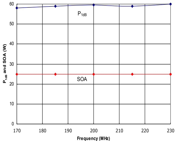
Figure 4: HD30723 Typical P 1dB and Safe Operating Area (SOA). The amplifier is capable of delivering much more power than it is safe to generate. Do not exceed the indicated SOA.
