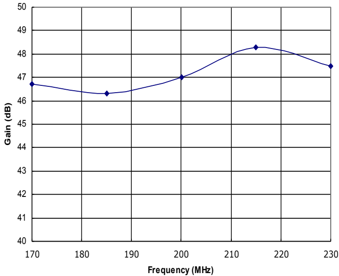
Figure 1: HD30723 Typical Gain @ P out = 25W.
