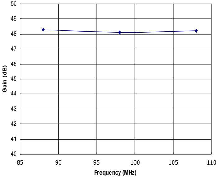
Figure 1: HD30721 Typical Gain @ P out = 25W.
