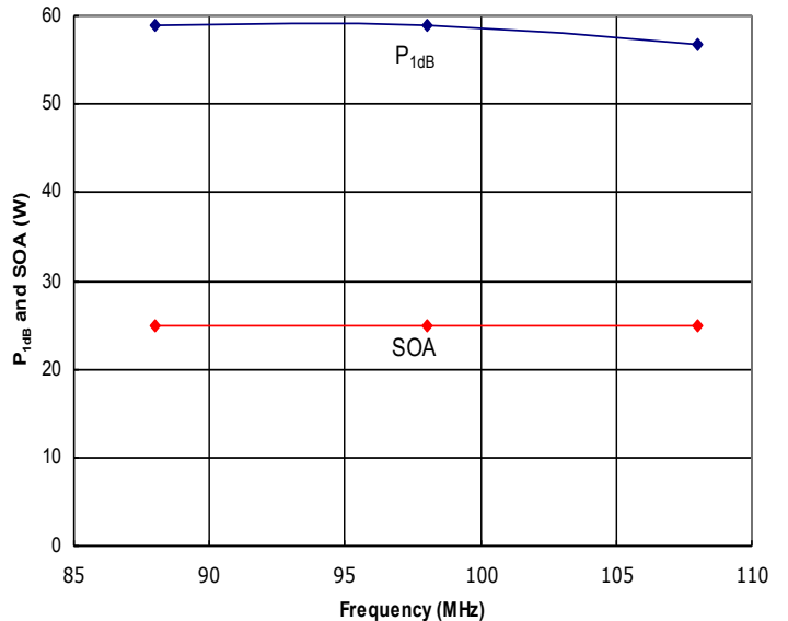
Figure 4: HD30721 Typical P 1dB and Safe Operating Area (SOA). The amplifier is capable of delivering much more power than it is safe to generate. Do not exceed the indicated SOA.
