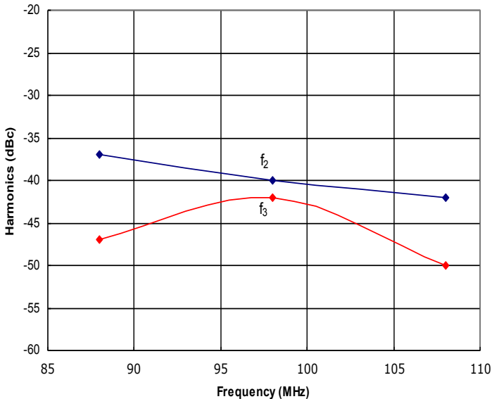
Figure 3: HD30721 Typical f 2 and f 3 @ P out = 25W.
