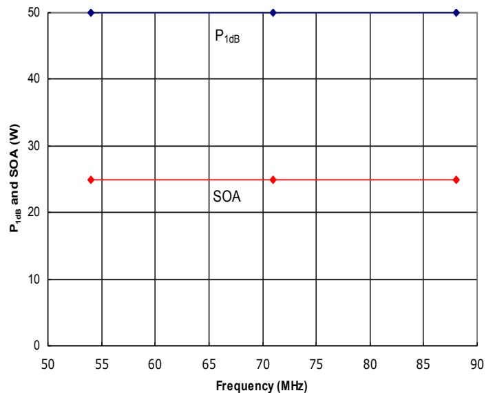
Figure 4: HD30720 Typical P 1dB and Safe Operating Area (SOA). The amplifier is capable of delivering much more power than it is safe to generate. Do not exceed the SOA shown above.
