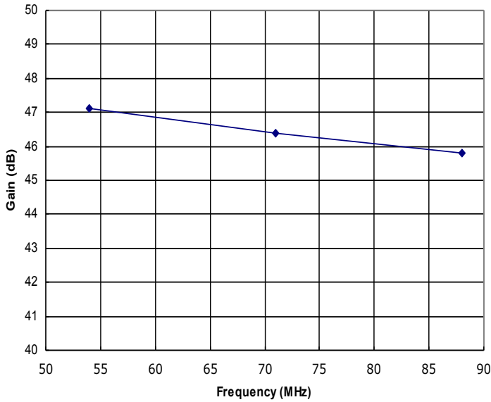
Figure 1: HD30720 Typical Gain @ P out = 25W.
