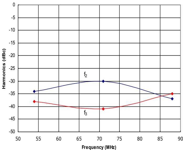
Figure 3: HD30720 Typical f 2 and f 3 @ P out = 25W.
