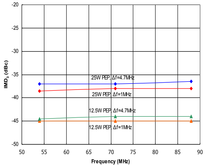
Figure 2: HD30720 Typical IMD 3 @ 25W and 12.5W PEP, Δf=1MHz and Δf=4.7MHz.
