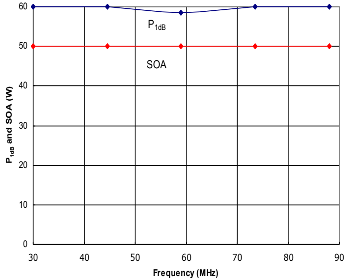
Figure 4: HD30719 Typical P_{1dB} and Safe Operating Area (SOA).
