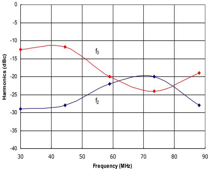
Figure 3: HD30719 Typical f_2 and f_3 @ P_{out} = 50W .
