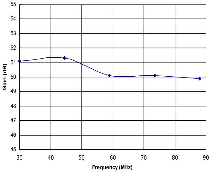
Figure 1: HD30719 Typical Gain @ P_{out} = 50W .
