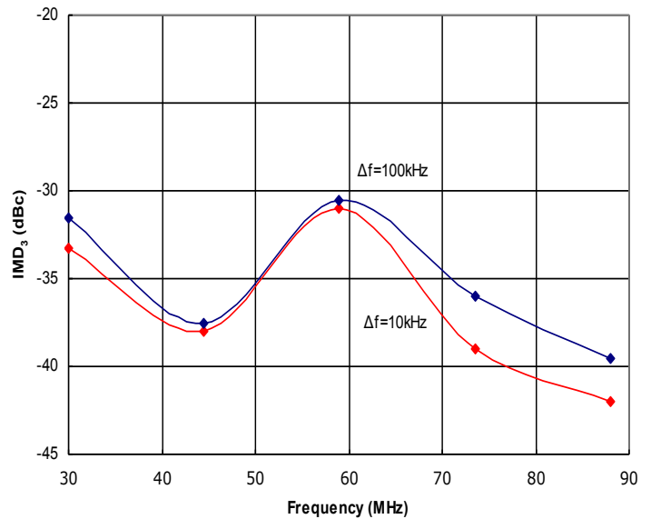
Figure 2: HD30719 Typical IMD_3 @ 50W PEP, \Delta f=10kHz and \Delta f=100kHz . For improved linearity, see our HD30718 Class A amp.
