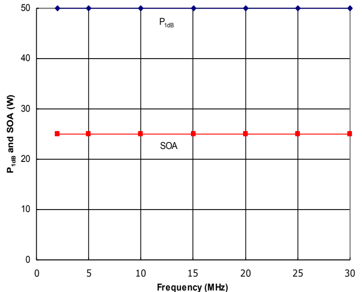
Figure 4: HD30716 Typical P 1dB and Safe Operating Area (SOA). The amplifier is capable of delivering much more power than it is safe to generate. Do not exceed the SOA shown above.
