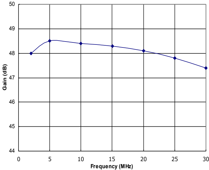
Figure 1: HD30716 Typical Gain @ P out = 25W.
