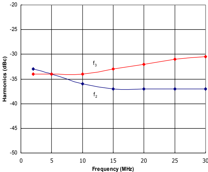
Figure 3: HD30716 Typical f 2 and f 3 @ P out = 25W.
