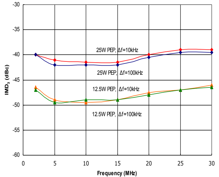
Figure 2: HD30716 Typical IMD 3 , @ 25W and 12.5W PEP, Δf=10kHz and Δf=100kHz.
