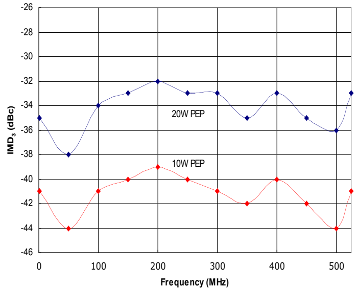
Figure 2: HD30706 Typical IMD_3 , \Delta f = 10kHz , @ P_{out} = 20W and 10W PEP.
