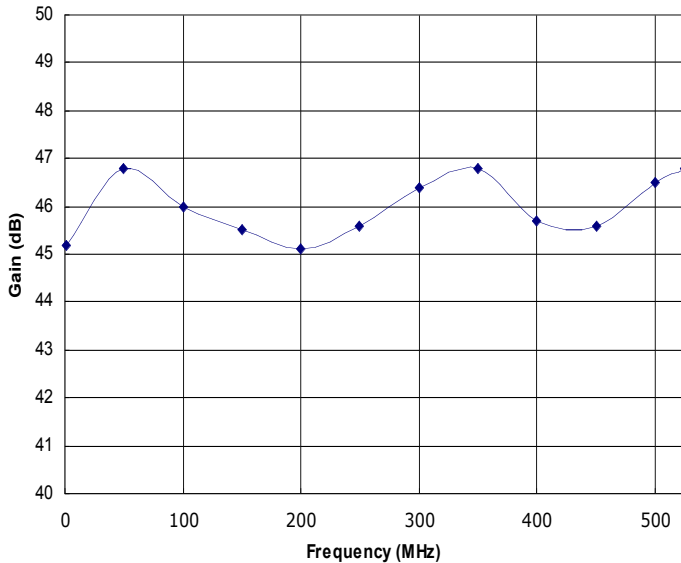
Figure 1: HD30706 Typical Gain @ P_{out} = 20W .
