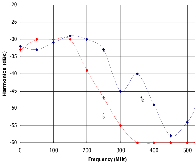
Figure 3: HD30706 Typical f_2 and f_3 @ P_{out} = 20W .
