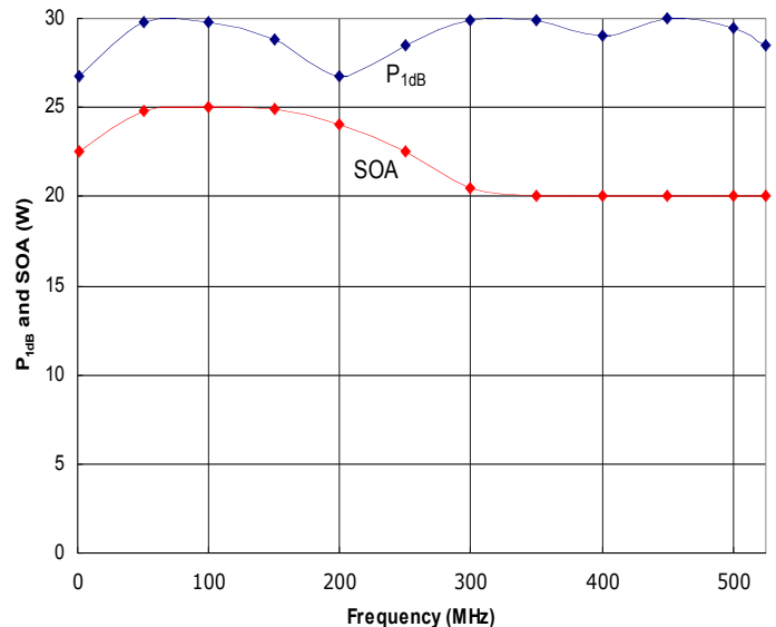
Figure 4: HD30706 Typical P_{1dB} and Safe Operating Area (SOA). The amplifier is capable of delivering more power than it is safe to generate. Do not exceed the SOA without first contacting HD to discuss your application.
