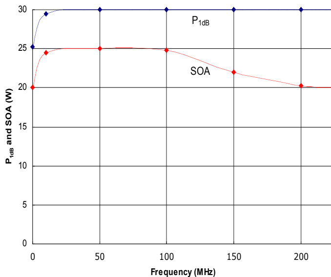
Figure 4: HD30664 Typical P 1dB and Safe Operating Area (SOA). The amplifier is capable of delivering more power than it is safe to generate. Do not exceed the SOA without first contacting HD Communications to discuss your application.
