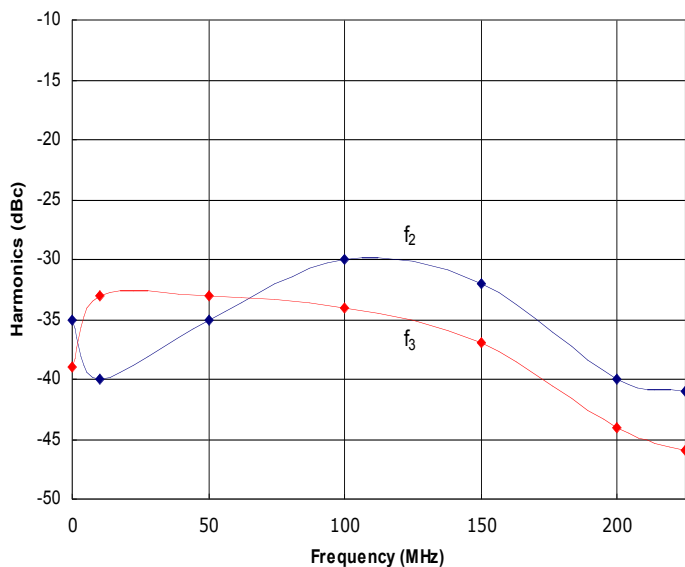
Figure 3: HD30664 Typical f 2 and f 3 @ P out = 20W.
