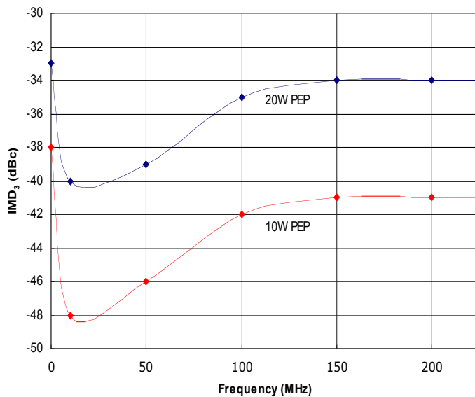
Figure 2: HD30664 Typical IMD 3 , Δf=10kHz, @ P out = 20W and 10W PEP.
