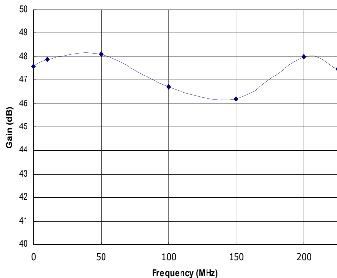
Figure 1: HD30664 Typical Gain @ P out = 20W.
