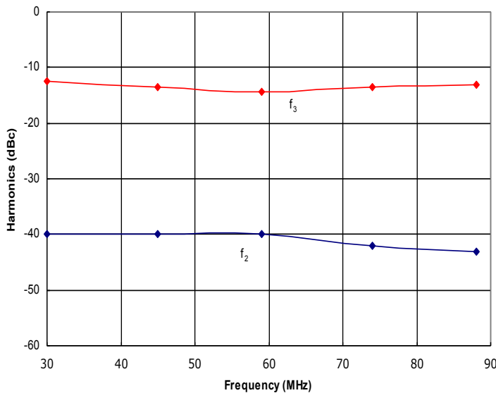
Figure 3: HD31584 Typical f 2 and f 3 @ P out = 350W.
