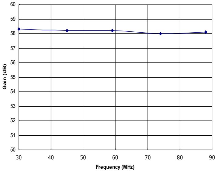
Figure 1: HD31584 Typical Gain @ P out = 350W.
