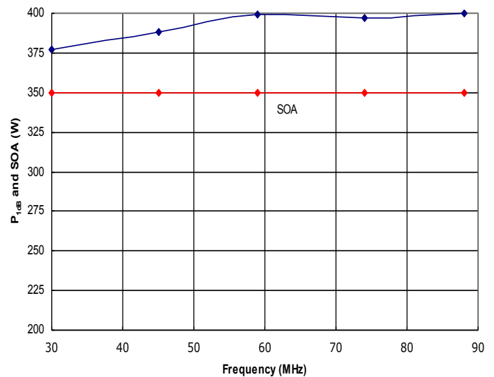
Figure 4: HD31584 Typical P 1dB and Safe Operating Area (SOA). The amplifier is capable of delivering more power than it is safe to generate. Do not exceed the SOA shown above without first contacting HD COMMUNICATIONS CORP. to discuss your application.
