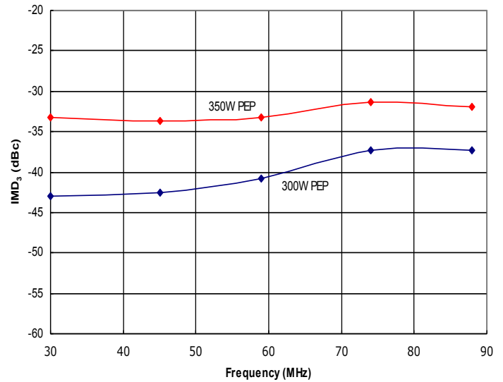
Figure 2: HD31584 Typical IMD 3 @ 350W and 300W PEP, Δf = 100kHz.
