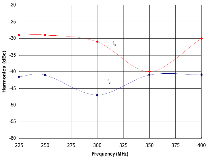
Figure 3: HD31371 Typical f 2 and f 3 @ P out =50W.
