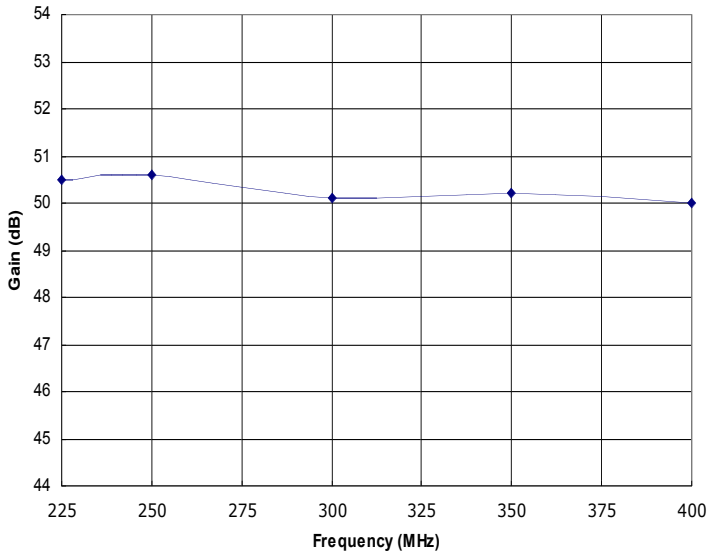
Figure 1: HD31371 Typical Gain @ P out =50W.
