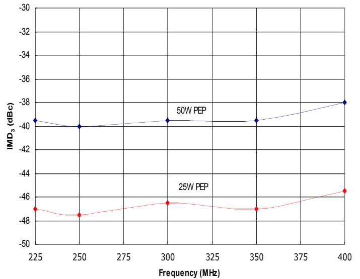
Figure 2: HD31371 Typical IMD 3 @ 50W and 25W PEP, Δf=10kHz and Δf=100kHz.
