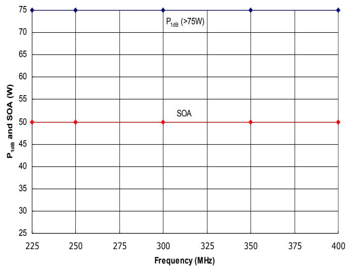
Figure 4: HD31371 Typical P 1dB and Safe Operating Area (SOA). The amplifier is capable of delivering much more power than it is safe to generate. Do not exceed the SOA shown above without first contacting HD Communications Corp. to discuss your application.
