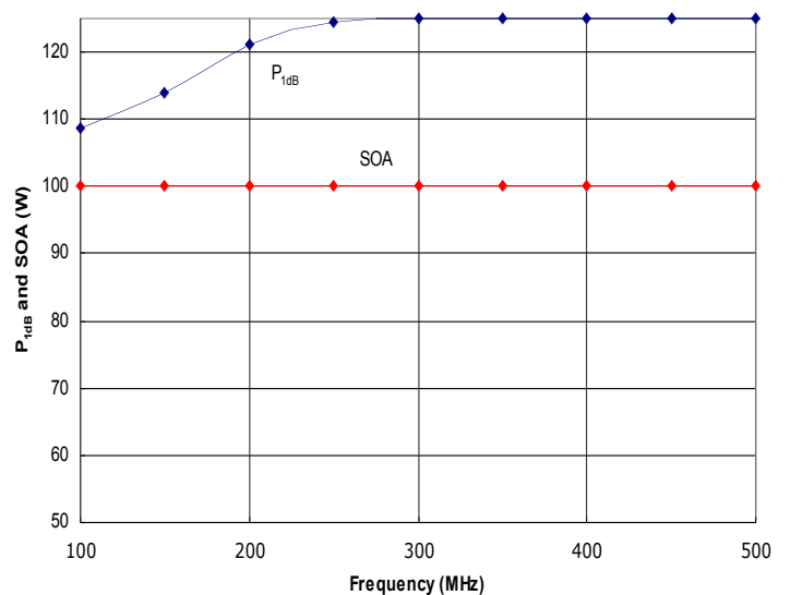
Figure 4: HD31348 Typical P 1dB and Safe Operating Area (SOA). Do not exceed the SOA shown above without first contacting HD Communications Corp. to discuss your application.
