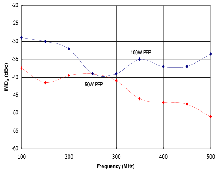
Figure 2: HD31348 Typical IMD 3 @ 100W and 50W PEP, Δf=10kHz. For improved linearity, see our HD31346 Class A amplifier.
