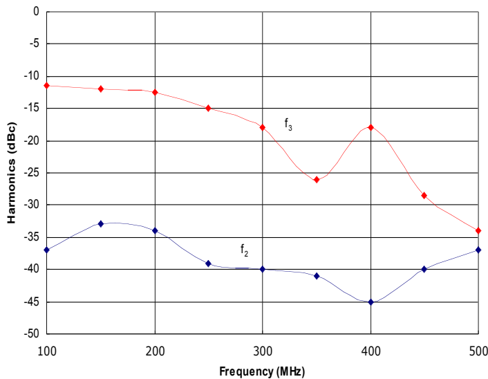
Figure 3: HD31348 Typical f 2 and f 3 @ P out =100W.
