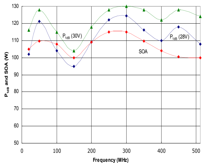
Figure 4: HD31344 Typical P_{1dB} @ 28VDC and 30VDC, and Safe Operating Area (SOA). Do not exceed the SOA shown above without first contacting RFMPT to discuss your application.
