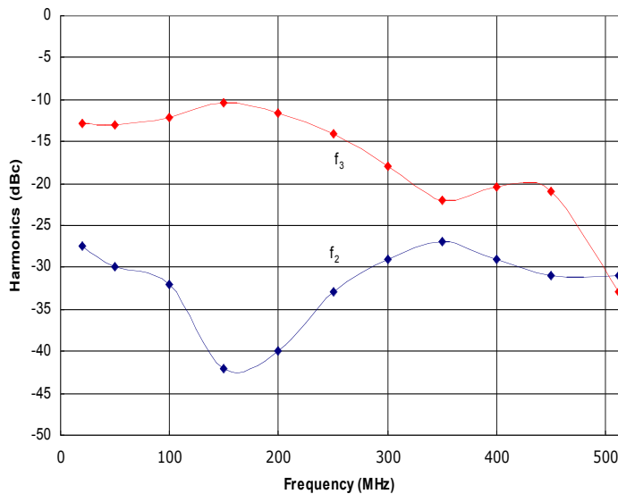
Figure 3: HD31344 Typical f_2 and f_3 @ P_{out}=100W .
